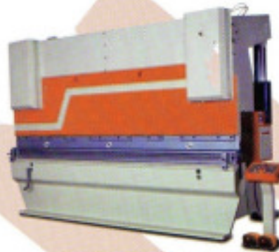
CNC / HYDRAULIC PRESS BRAKE S Available in Sizes : 1500 X 1.6mm - 4000 X 12mm
