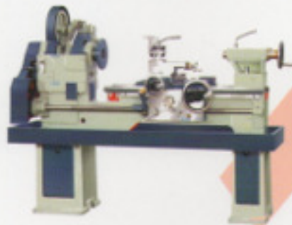
MEDIUM DUTY LATHE MACHINE "V" BELT & NORTON GEAR BOX TYPE Available in Sizes 4 1/2', 5 1/2' & 6'
