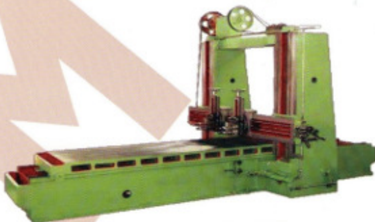
HEAVY DUTY PLANNER/PLANNO MILLER Available in Size From 4" to 20"
