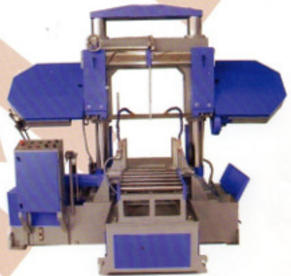
FULLY AUTOMATIC DOUBLE COLUMN HORIZONTAL BANDSAW
