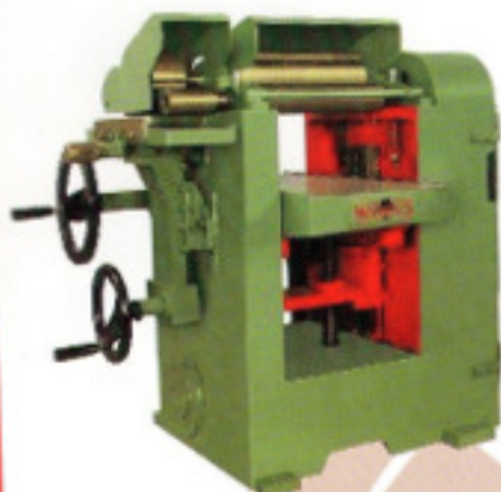
CLASSIC SERIES THICKNESS PLANNER - Screw Type
