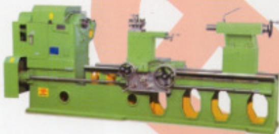
ROLL TURNING LATHE MACHINE EXTRA HEAVY DUTY PLANNER BEAD "V" BELT DRIVE Available in Sizes 12' - 30'
