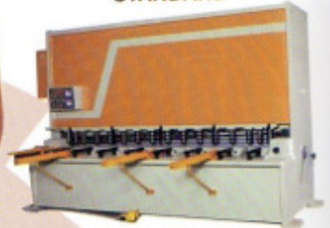
HYDRAULIC SHEARING MACHINE / CNC Available in Sizes : 1250 X 4mm - 6000 X 25mm
