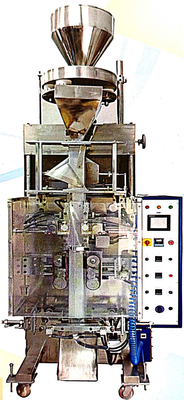
Automatic VFFS (Collar Type) machine for four corner seal (Quad) Pouch with volumetric cup filler (Model No. : CTQ 500+CF)
