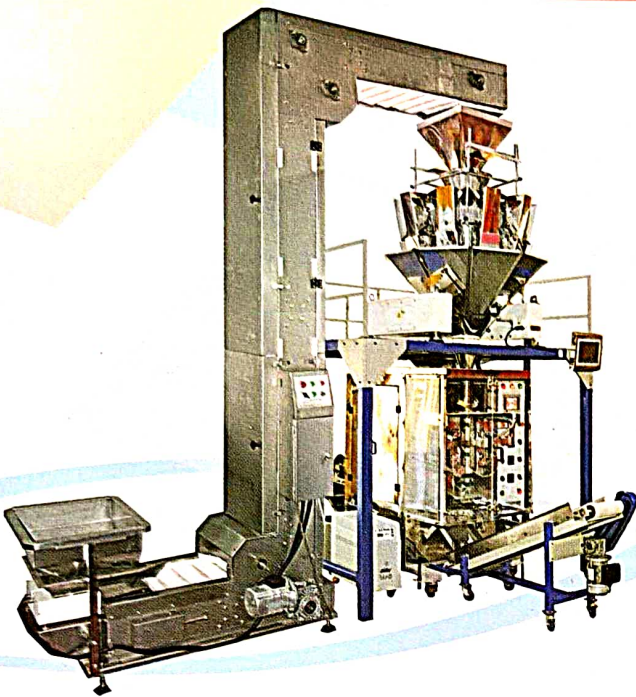
Automatic VFFS (Collar Type) machine with Multihead Combination weigh filler & Infeed Conveyor (Model No. - CT 500 + JW + IC-Z)
